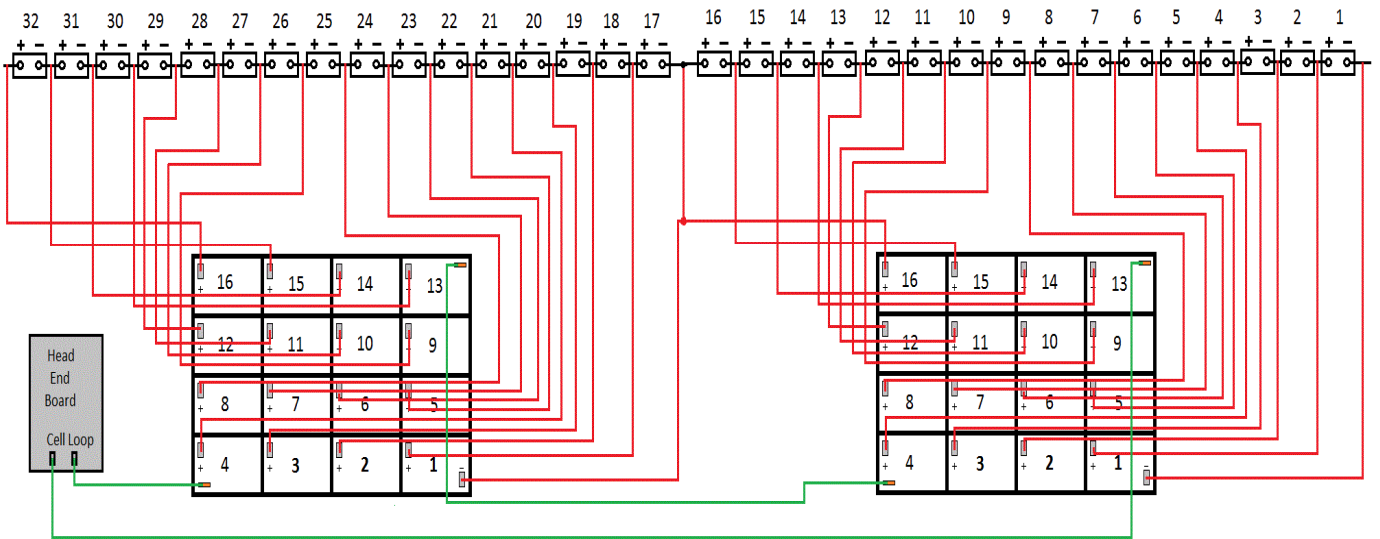
MiniBMS Centralized Installation Diagram
